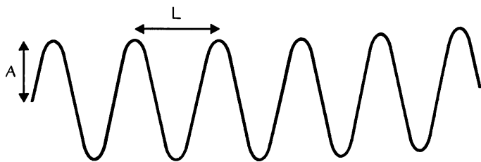
a wave pattern
