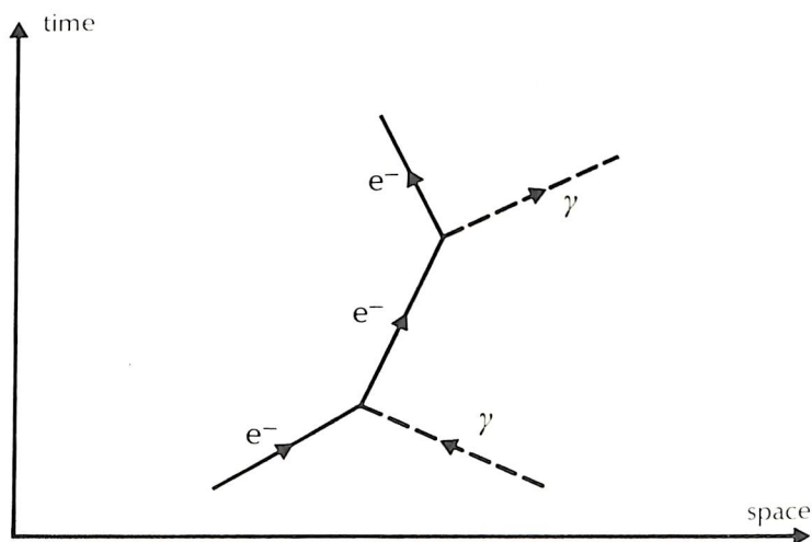
electron-photon scattering
