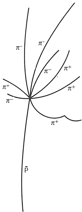
Creation of eight pions in a collision between an antiproton ( \bar{p} ) and a proton (sitting in the bubble chamber); see photograph on preceding page
