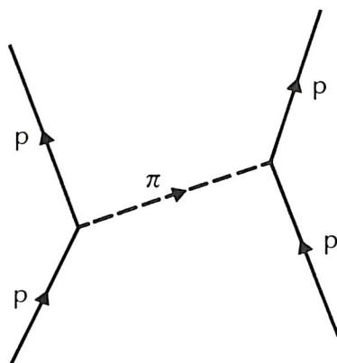
exchange of a pion ( \pi ) between two protons ( p )
