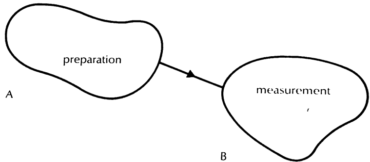
observation of a particle in atomic physics
