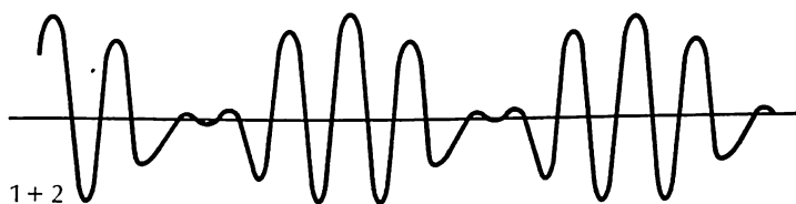
interference of two waves
