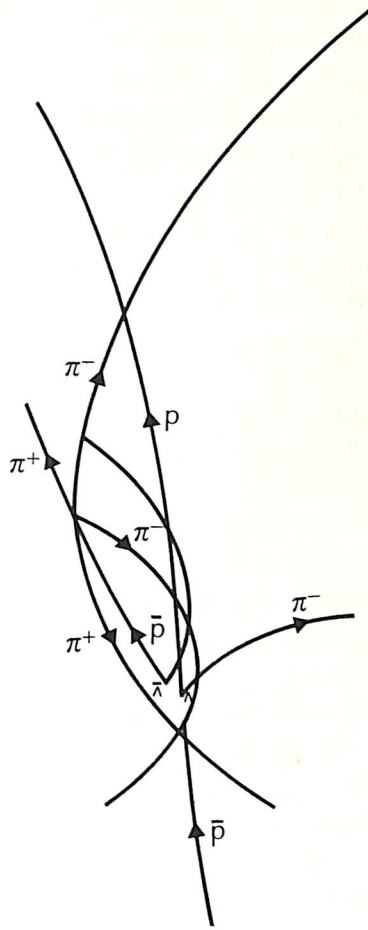
a network of reactions involving protons, antiprotons, a lambda-antilambda pair, and several pions
