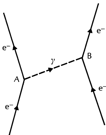
mutual repulsion of two electrons through the exchange of a photon
