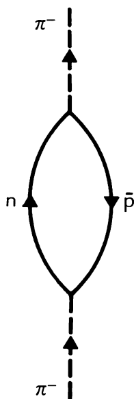
creation of a virtual neutron-antiproton pair
