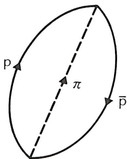
a vacuum diagram
