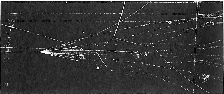
creation of sixteen particles in a pion-proton collision
