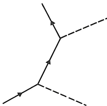
electron-photon scattering
