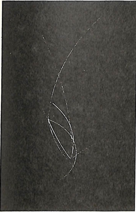
a network of reactions involving protons, antiprotons, a lambda-antilambda pair, and several pions
