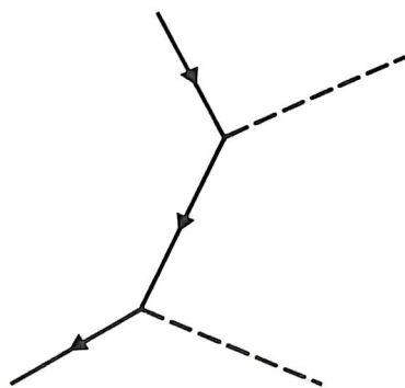
positron-photon scattering
